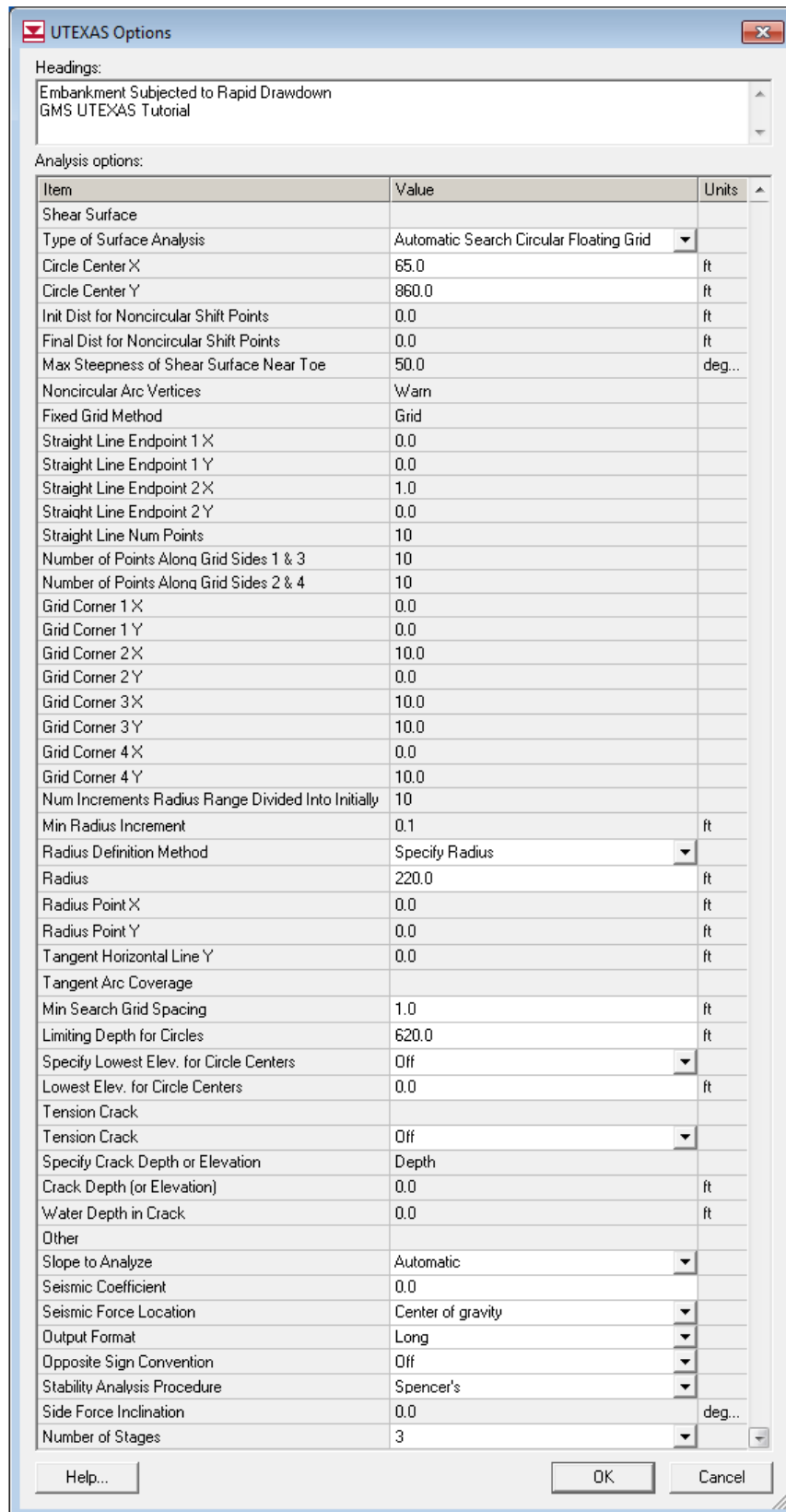
Figure 3 UTEXAS Options
